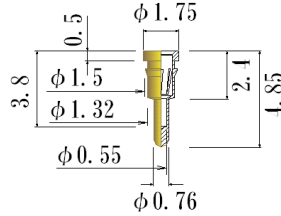
Acceptable plug: \phi 0.60 \sim \phi 0.40 JS0041-1L-GG
