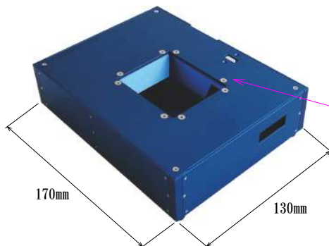
Mounting Socket
